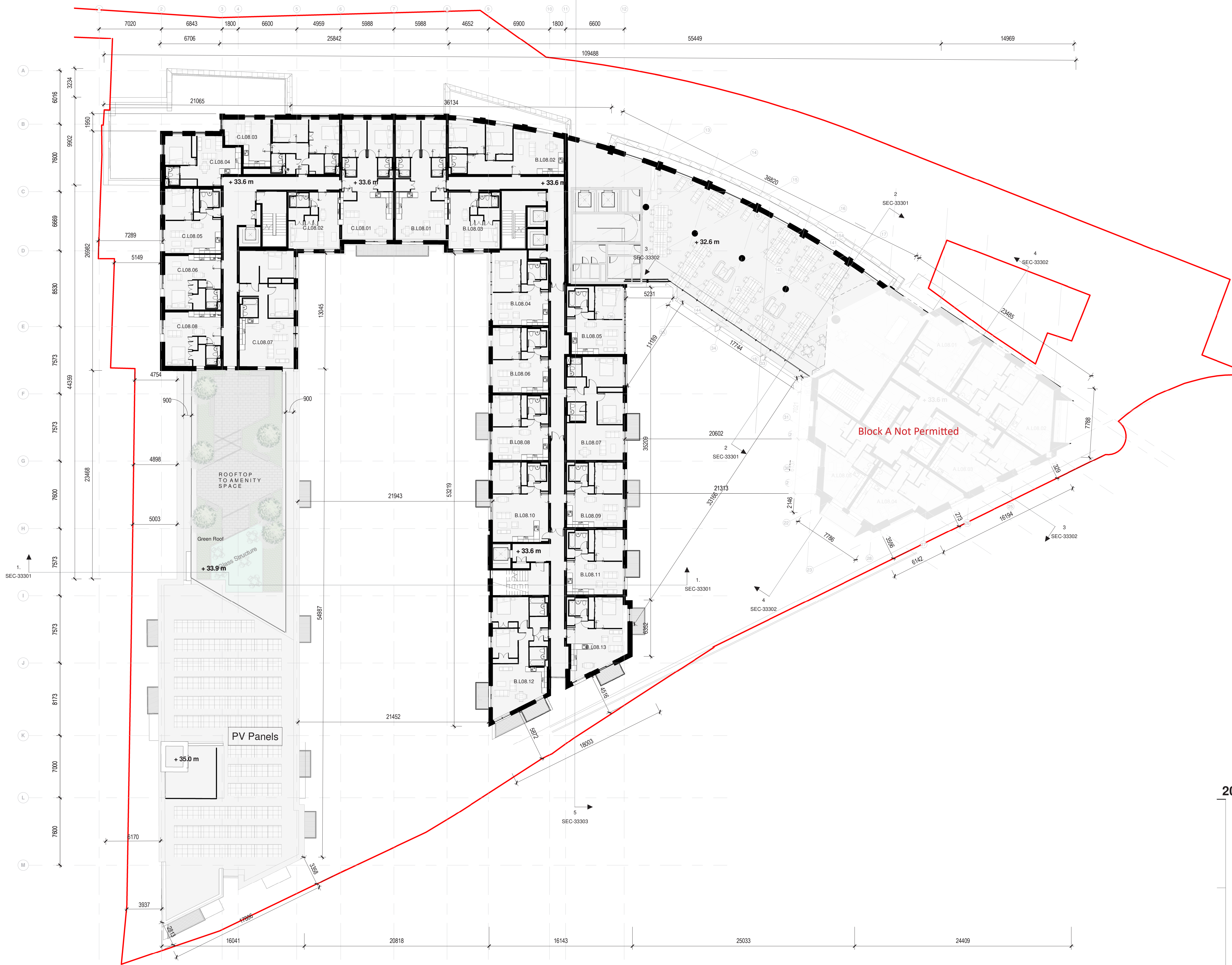
Proposed 8th Floor Plan 1 : 200
